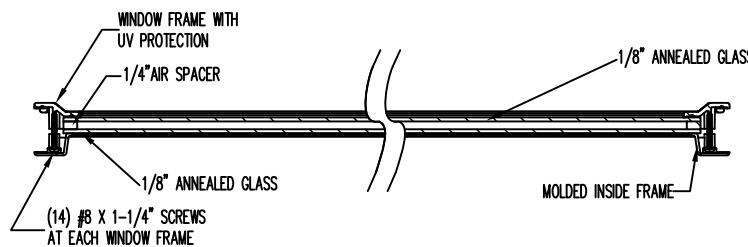
SECTION C-C
