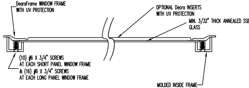
SECTION B-B
